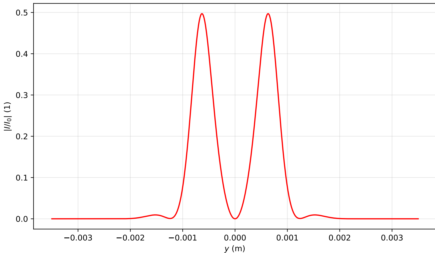
Intensity profile I(x=0, y, z=1.353)/I_0 , P_{in}=5.0P_{cr} , artificial time
